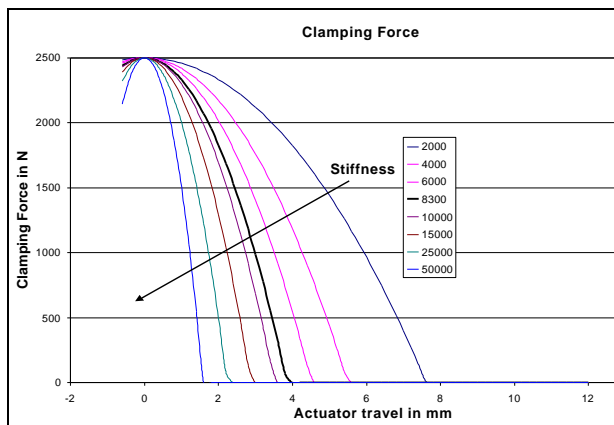
Figure 6: Clamping Force
