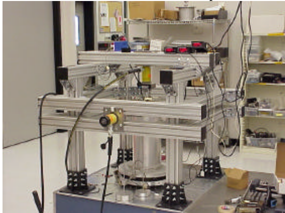
Figure 10. Clamp band system assembled in structural test fixture.
