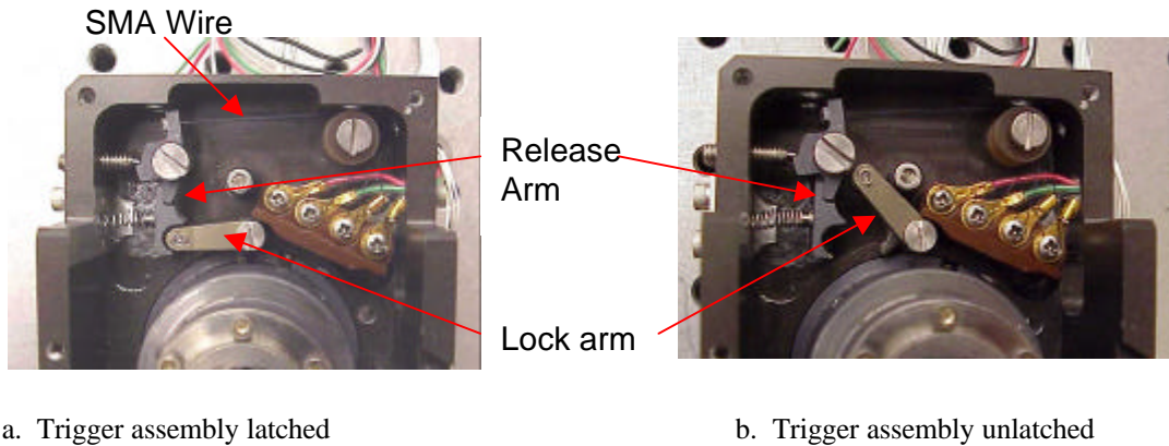
Figure 6. Two views of the SMA trigger assembly showing major components.
