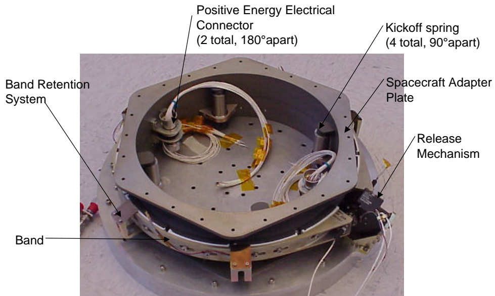
Figure 3. Clamp band system with major components identified. System is shown in clamped, preloaded configuration.
