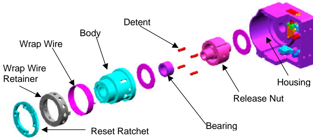
Figure 4. Release mechanism detail view.
