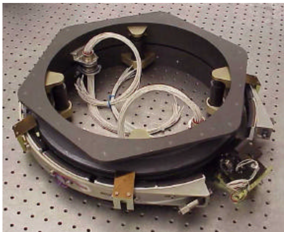
Figure 2. Nanosat configuration of clamp band system.
