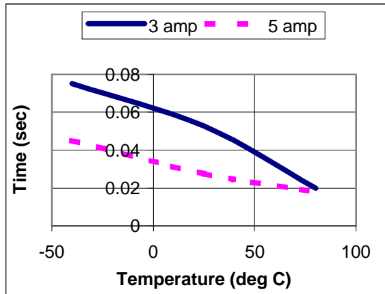
Figure 8. Release time dependence on applied current and environmental temperature.
