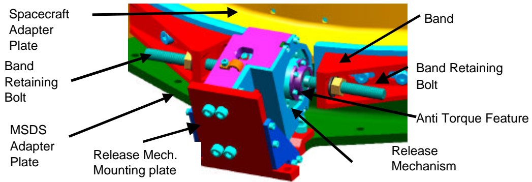
Figure 4. Release mechanism detail view.
