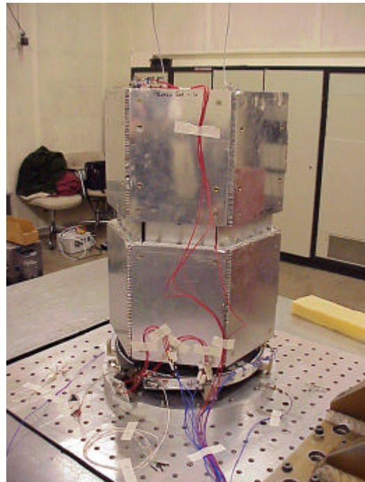
Figure 11. Stanford mass simulator supported by clamp band system on vibration table.
