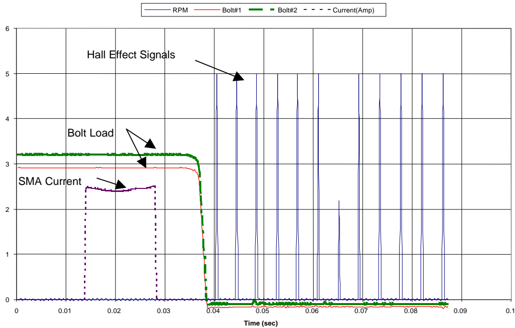
Figure 7. Typical functional data from functional test of release system. Data is for 25°C, 5 Amp operation.
