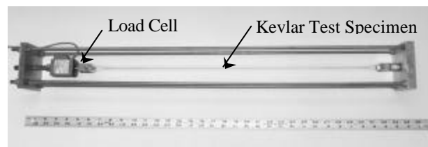
Figure 11: Test Specimen Load Relaxation Test Fixture
