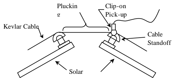
Figure 10: Musical Pick-up Attachment to Cable Standoff on Spacecraft, 1 of 4 Locations
