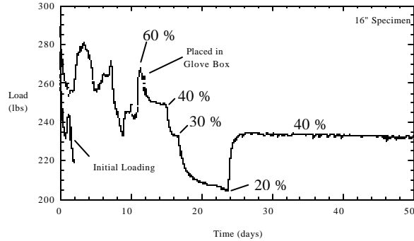
Figure 12: Load Over Time With Varying Relative Humidity
