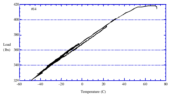
Figure 16: Load versus Temperature
