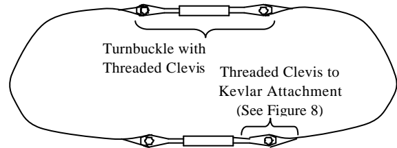
Figure 7: Kevlar Cable Assembly with Turnbuckle
