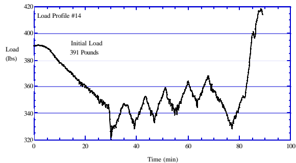
Figure 15: Cable Load Based on Temperature Profile
