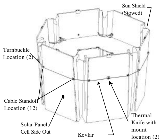
Figure 2: Stowed Configuration (Instrument not shown)
