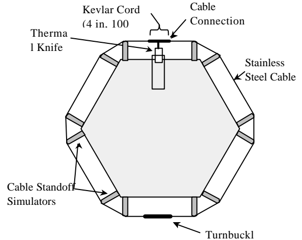
Figure 5: Top View, Prototype Testing Setup
