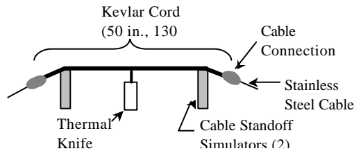
Figure 6: Extended Kevlar Section
