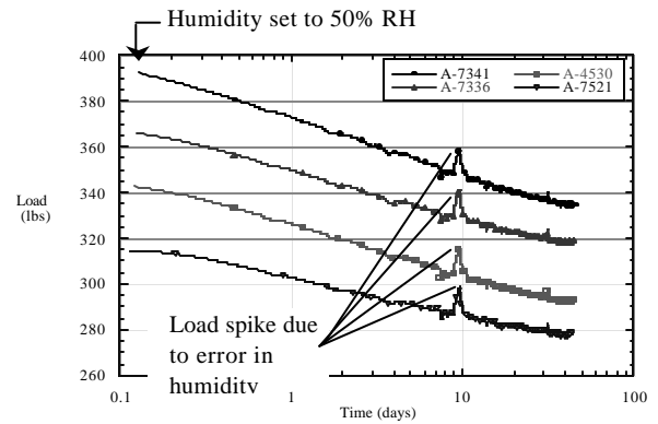
Figure 13: 45-Day Cable Relaxation Rate
