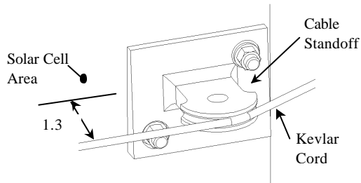
Figure 3: Cable Standoff with Kevlar Cord
