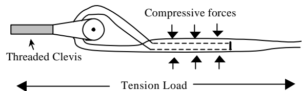
Figure 8: Kevlar to Turnbuckle Attachment
