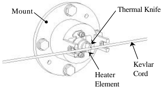
Figure 4a: Thermal Knife in Mount
