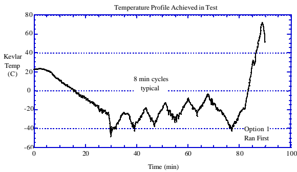
Figure 14: SARRS Cable Temperature Profile
