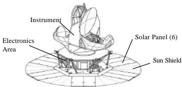
Figure 1: MAP Spacecraft in Deployed Configuration
