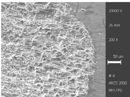
Fig. 14 Surface of disc SS17-7ph with MoS 2 coating after fretting tests (compare to Fig. 11 for adhesion forces): lubrication effect was lost after less than 200 second fretting movement (confirmed by EDAX-mapping: no Mo present in contact area).
