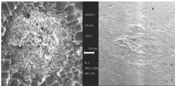
Fig. 15 Comparison of Al-coatings under fretting: Left: Hard anodising on Al7075 was broken. Right: Keronite coating on Al AA 2219 does not show fretting marks. (Compare to Fig. 11 for adhesion forces).
