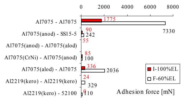
Fig. 12 Adhesion force of aluminium based coatings (I=impact and F=fretting): Adhesion between Al parts is strongly reduced by hard anodising (anod), CrNi-plating (CrNi) and Keronite [10],[12]. A single Alodine coating (alod) is not efficient in prevention of cold welding.
