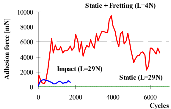
Fig.2 Adhesion force as function of cycles (i.e. one closing-separation) [1]. Comparison of adhesion in static (load 29N), impact (load 29N) and fretting (load 4 N) condition under vacuum. Danger and severity of adhesion increases with type of contact: static- impact – fretting. (Max. adhesion in static 0.1 N after > 25,000 cycles, in impact 0.96 N, in fretting 9.5 N.)
