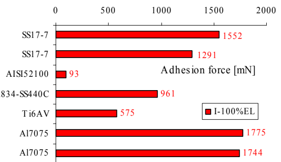
Fig.4 Adhesion force under impact for materials in contact to themselves. Highest adhesion for stainless steels with Nickel (e.g. SS17-7PH), Inconel, Titanium alloys (IMI834) and Al alloys (Al AA7075). Low adhesion for bearing steel AISI 52100 (no Ni).
