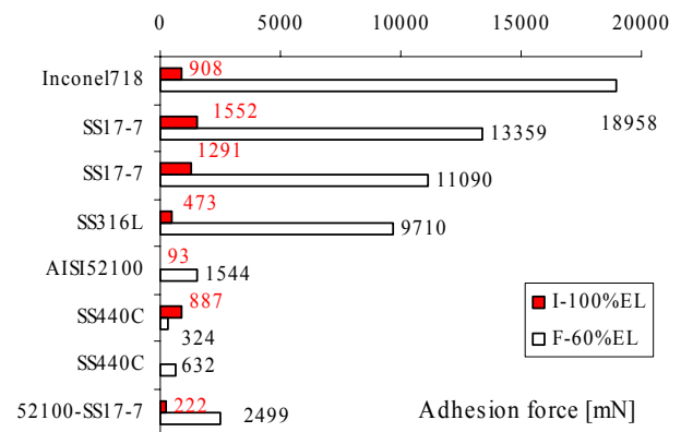
Fig.10 Comparison of adhesion force under impact (I) and fretting (F) for different steels and Ni-alloys versus themselves: Adhesion under fretting decreases with decreasing content of Ni as indicated by [7]. Combinations of different steels seem to be dominated by the one with higher adhesion: AISI52100 to SS17-7ph. (52100-SS17)
