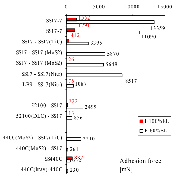
Fig. 11 Adhesion force of steel based coatings (I=impact and F=fretting): coatings in general reduce adhesion. For SS17-7PH no tested coating of the disc could decrease adhesion significantly (TiC, MoS 2 or nitriding). In contact of AISI440C to SS17-7ph, TiC shall be avoided. Efficiency of grease (Braycote601) is not significant in contact of AISI440C to itself. Efficiency of MoS 2 coating under fretting is limited to a low endurance.
