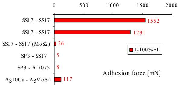
Fig.8 Adhesion force under impact for different combinations with MoS 2 :coatings and composites provide good prevention of cold welding (SP3 = Vespel SP3, Ag10Cu = coin silver, AgMoS 2 = silver composite with 15% MoS 2 ).
