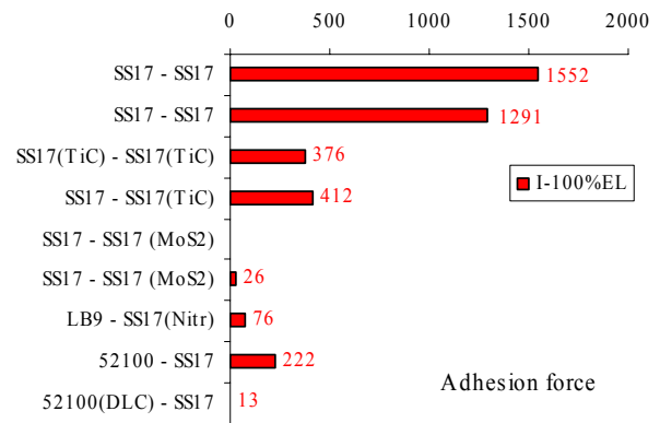
Fig.6 Adhesion force as function of static load for different coatings on steel: lowest adhesion for SS17-7PH (SS17) with MoS 2 . Higher adhesion for TiC (coatings was broken). Negligible adhesion between bronze (LB9) and SS17-7PH (LB9-SS17(Nitr)). Low adhesion between AISI52100 and SS17-7PH, can further be decreased by use of DLC coating (“52100(DLC)-SS17”).
