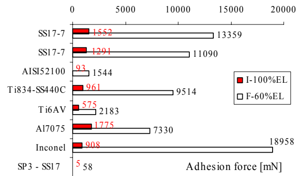
Fig.9 Comparison of adhesion force under impact (I) and fretting (F): Adhesion between metals under fretting are up to tenfold higher than under impact. Highest adhesion for Ti, Al-alloys, stainless steels containing Ni and Ni alloys (Inconel 718). No adhesion between polymer composite (VESPEL SP3: Polyimide with 15% MoS 2 ) and steel (SS 17-7PH).
