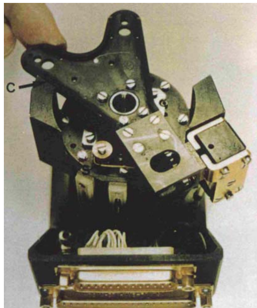
Fig. 1 Mechanism of a satellite: anchor was actuated from its resting position (middle) electromagnetically. It impacted on both end stops. Finally, an anomaly from the satellite was reported, that the anchor kept blocked on the left side. It was “cold welded”.
