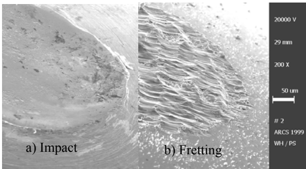
Fig. 13 Surface of a pin (SS17-7ph) after impact and fretting. Impact: only some plastic flow visible by piling up of edges. Fretting: strong destruction of surface, adhesive wear combined with high adhesion forces (Compare to Fig.10 for adhesion forces: “SS17-7”).
