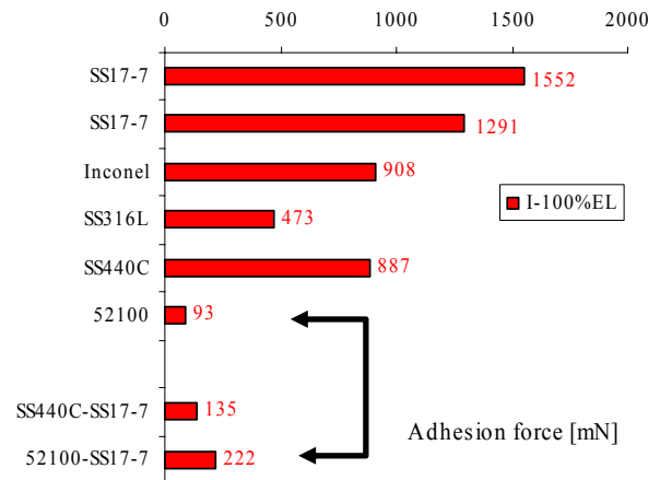
Fig.5 Adhesion force under impact for different types of steel versus itself: austenitic structure and Ni seem to promote high adhesion: SS17-7ph (7%), AISI 316L (11%), Inconel 718 (52%). No adhesion for AISI52100 versus itself ("52100"). High adhesion of AISI440C has to be proven. Combinations of different steels: adhesion seems to increase in contact to steels with higher tendency to cold welding (arrow).
