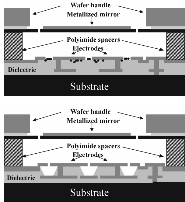
Figure 2 (from [16]). Top: a simpler geometry that is susceptible to performance degradation due to trapped charge. Bottom: improved geometry with selective etch to remove dielectric so that device performance is no longer affected by trapped charge.
