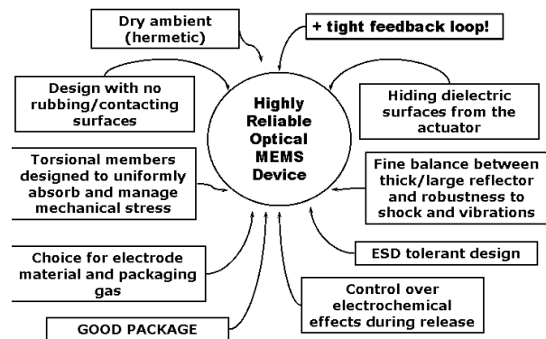
Figure 1. Schematic diagram of good design practices for electrostatically operated MOEMS devices. Most of the rules (in particular packaging and concurrent design) are applicable to all MEMS technologies.
