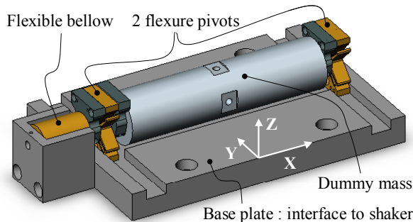
Figure 6: Vibration test bench
