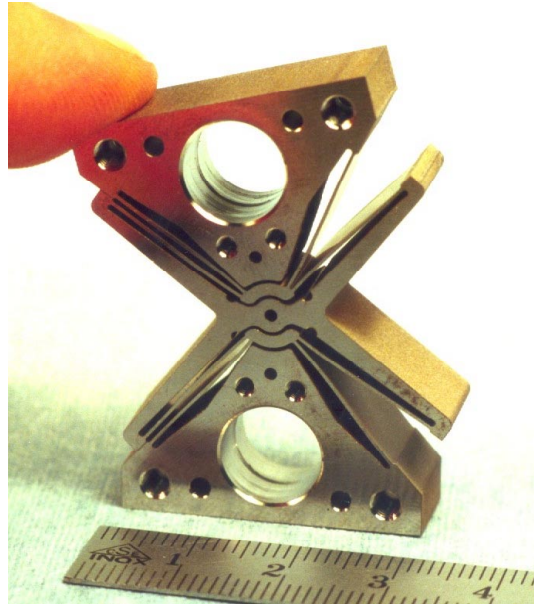
Figure 1: Picture of the monolithic "butterfly" flexure pivot. Angular stroke up to \pm 15^\circ . Parasitic translation (centre shift) below 2 \mu\text{m} for \pm 10^\circ strokes. Machined monolithically in Titanium.
