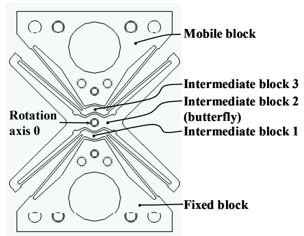
Figure 3: The "butterfly" pivot structure
