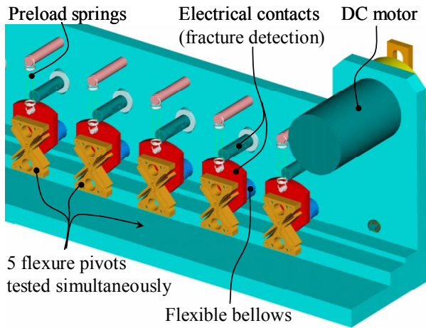
Figure 5: Fatigue test bed
