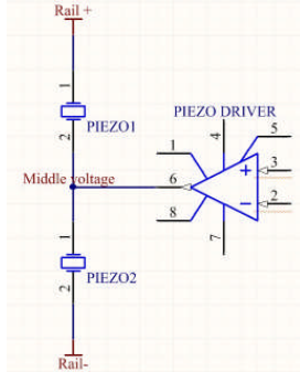
Figure 2. Electrical configuration for push-pull mechanisms.
