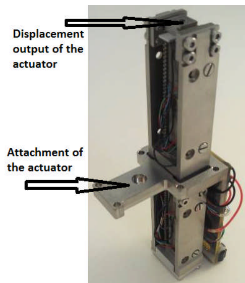
Figure 1. PPA40M-SG-based push-pull space-compliant mechanism.
