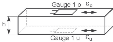
Figure 3. SG mounting on the ceramics.
