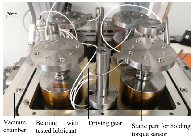
Figure 1. InS four bearings vacuum test bench
